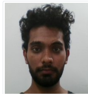
Captured
